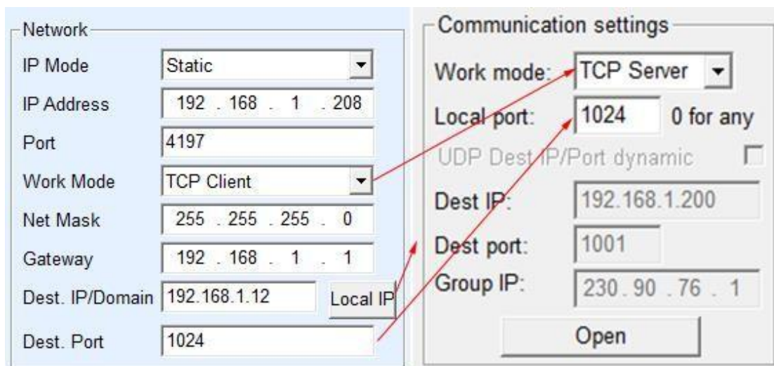
Figure 16 The serial port server as the Client
