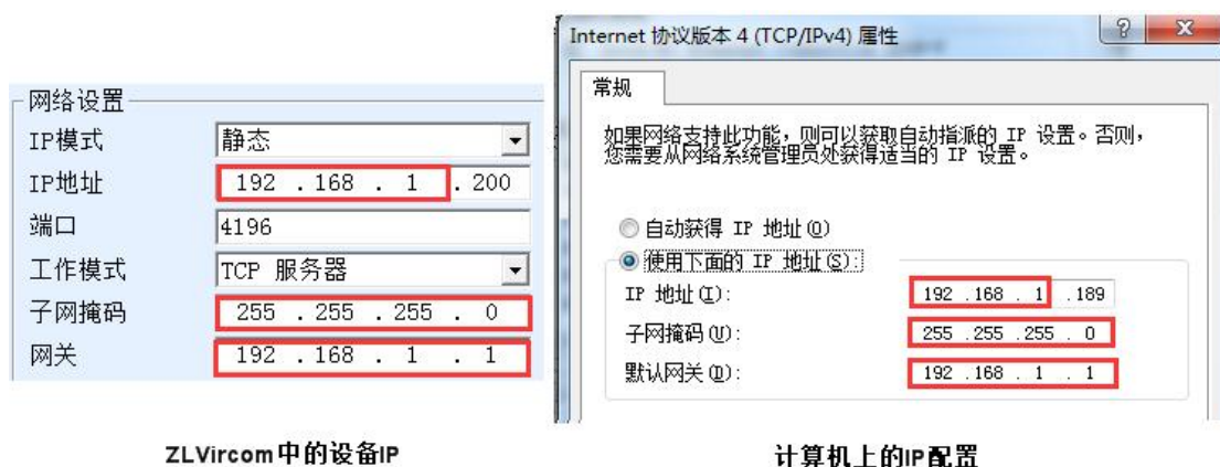
Figure 22 Configure on the same network segment
