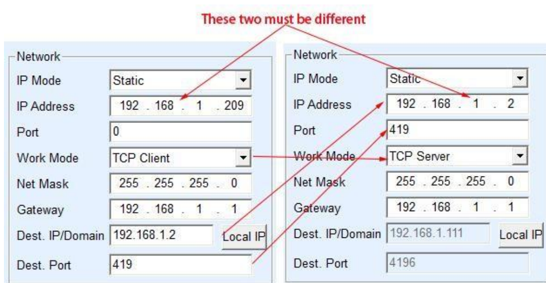
Figure 19 TCP device pairing parameter configuration
