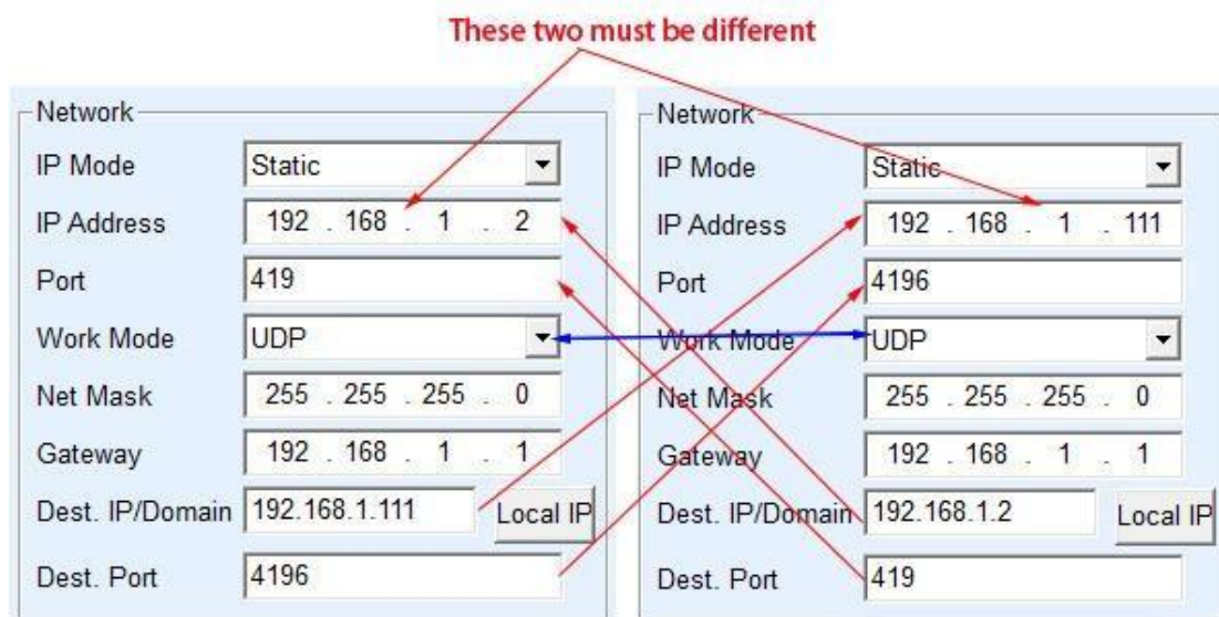
FIG. 21 configuration of UDP device pairing parameters
