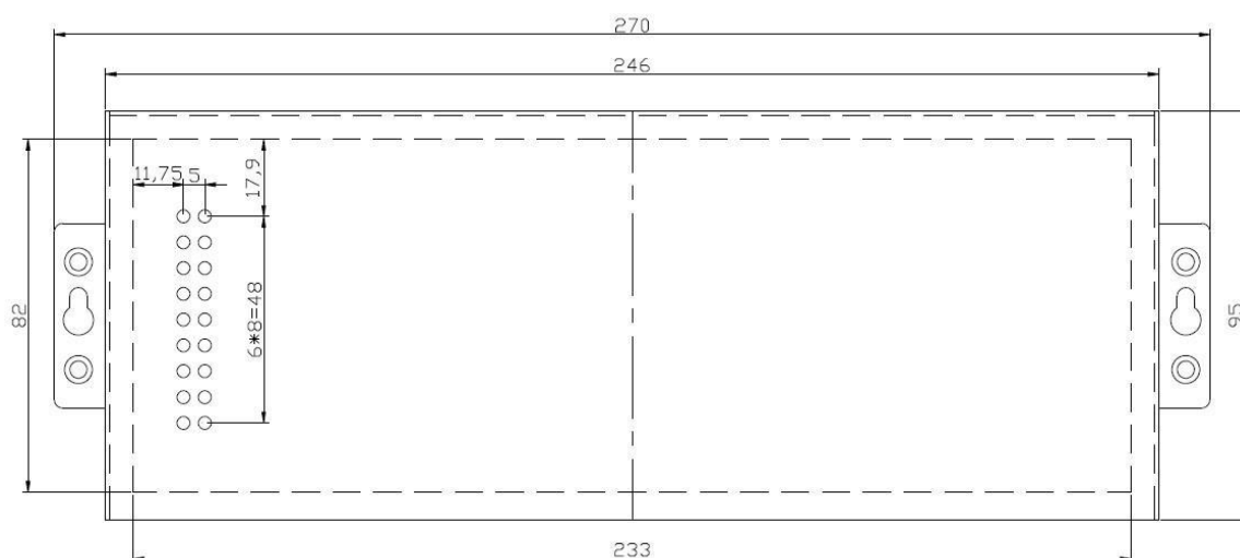
Figure 34 ZLAN5840I installation size
