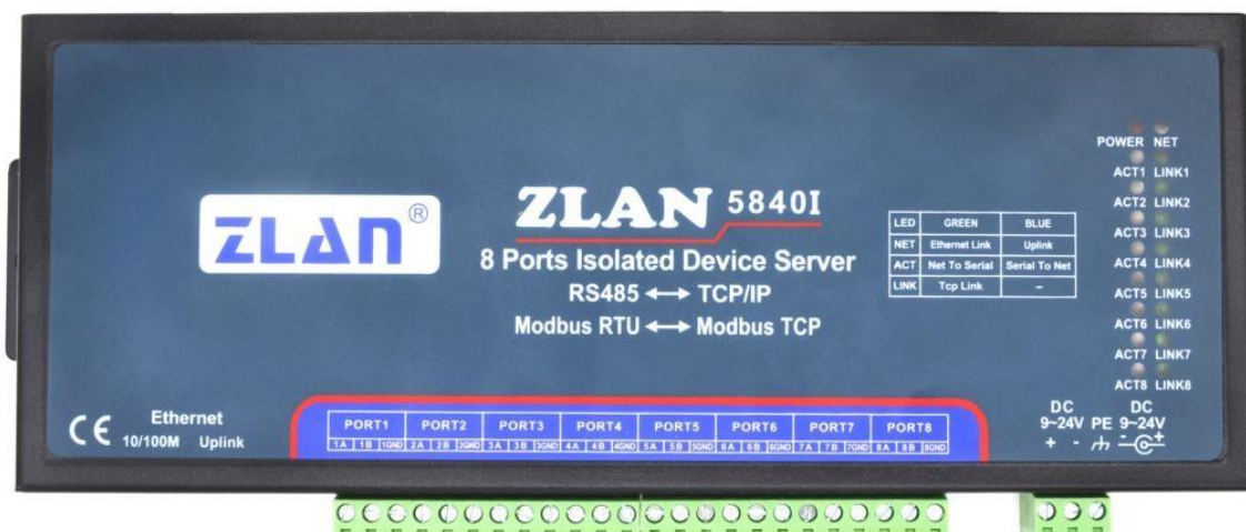
Figure 2 ZLAN5840I Front View
