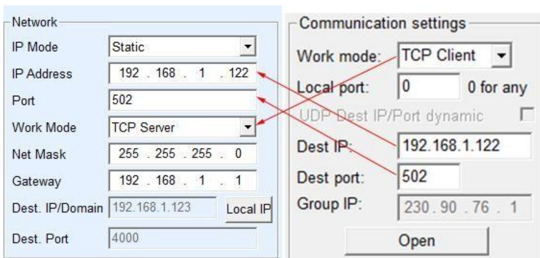
Figure 17 The serial port server as the Server
