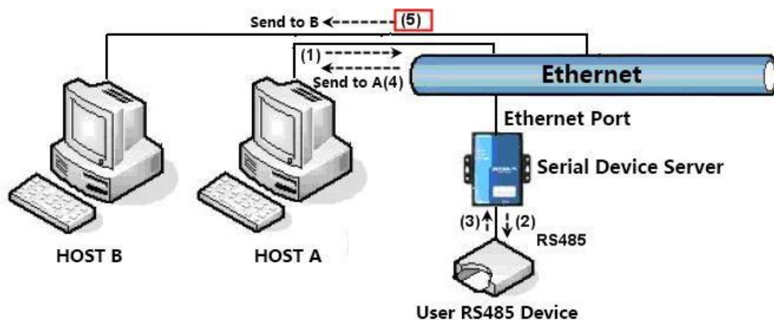
Figure 27 multi-host function demo
