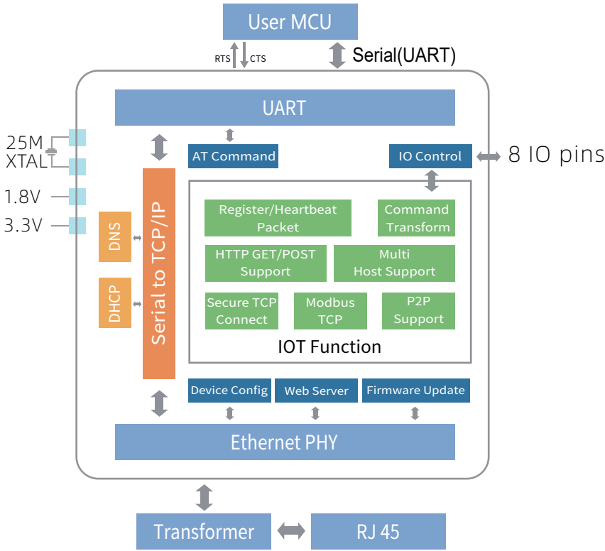
ZLAN1003 Block diagram
